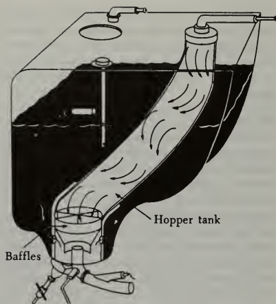
FIGURE 6-3. Oil tank with hopper.
